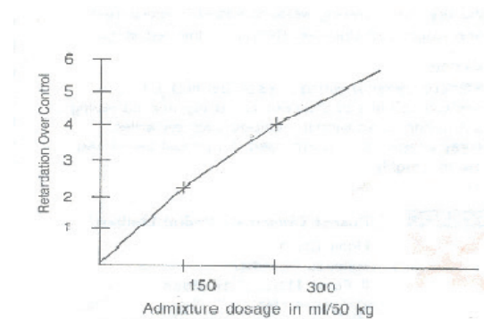
Conplast RP264 retardation Vs. Dosage at constant water content
